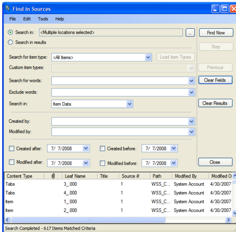
Figure 3-4. Find in Sources window with results
