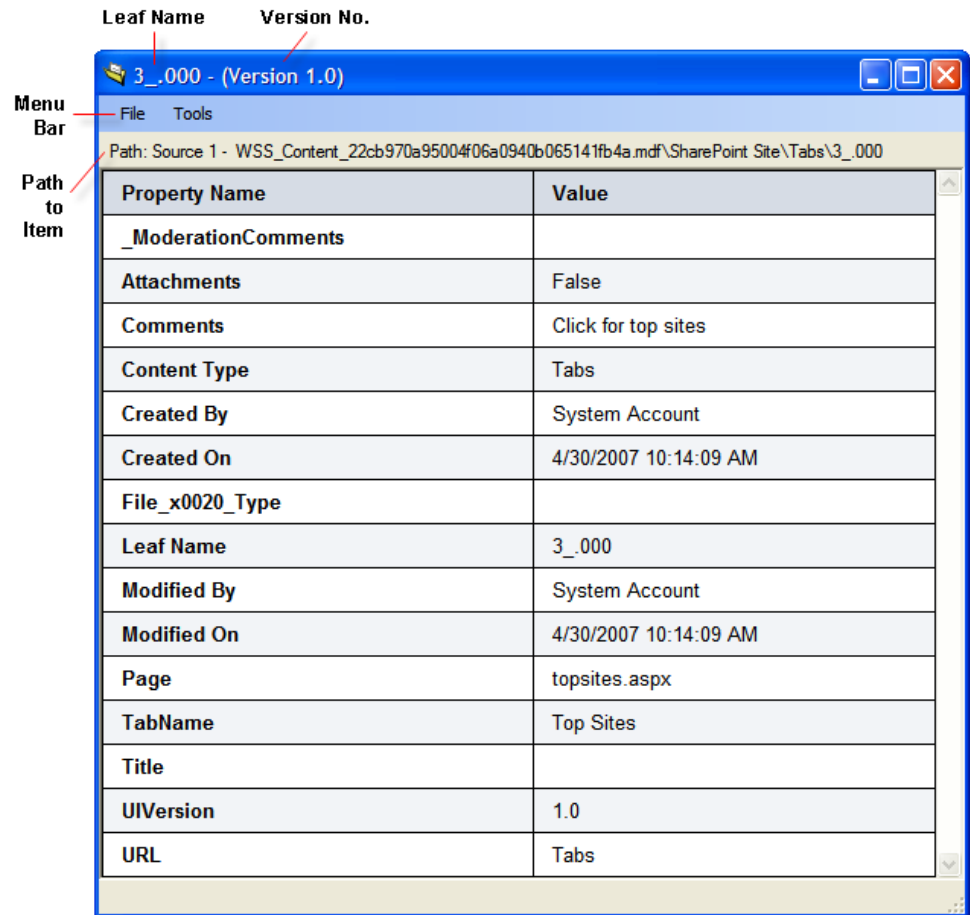
Figure 2-5. Metadata for an item
